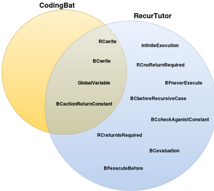
Fig. 7. Misconceptions covered by CodingBat and RecurTutor
