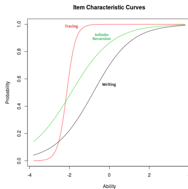
Fig. 8. Item response curves for the questions used to measure student performance on recursion
