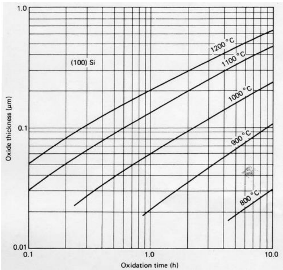
Oxide growth rate for dry oxygen
