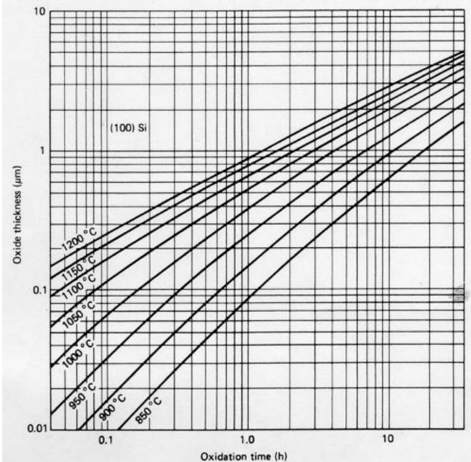
Oxide growth rate for wet oxygen
